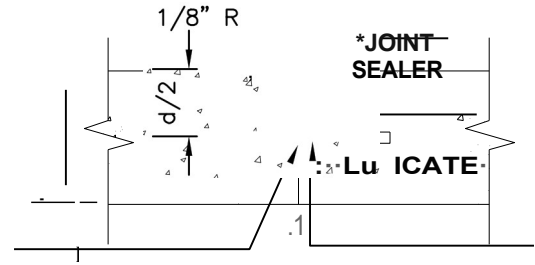
BUTT JOINT FORMED BULK HEAD
