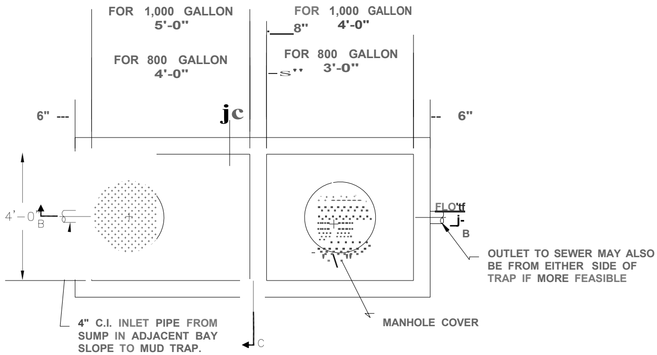
@ PLAN - GREASE TRAP TANK
