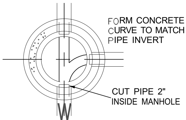
TYPICAL INVERT FOR PIPE INTERSECTIONS
