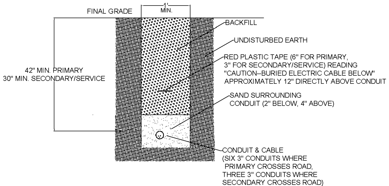
TRENCH DETAIL
