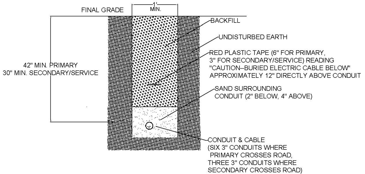
TRENCH DETAIL
