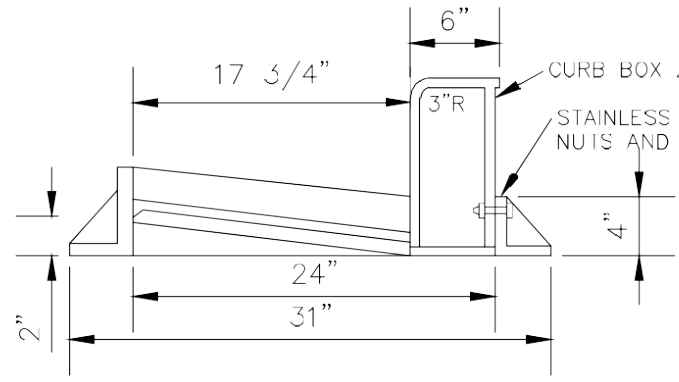
SECTION B-B
